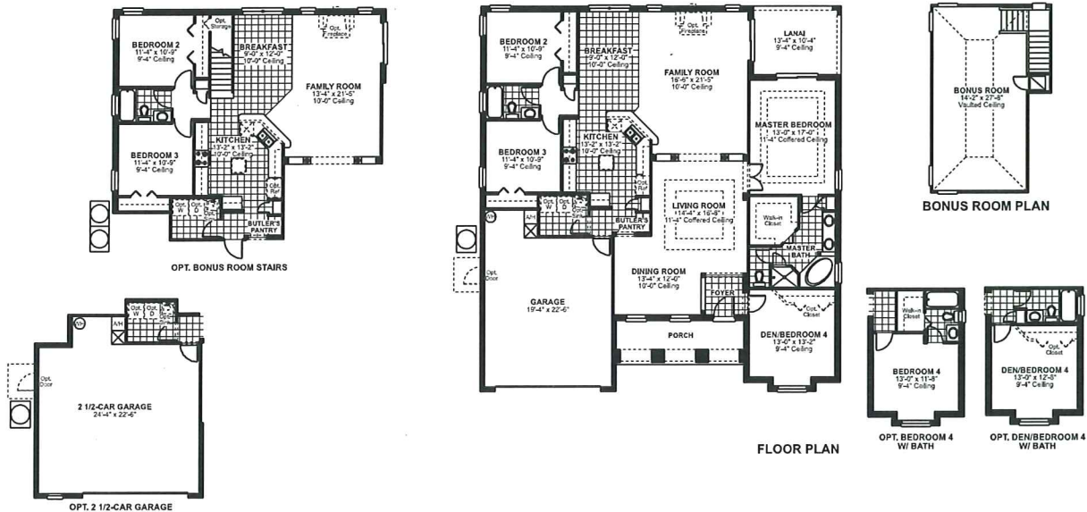
BROOKHAVEN II - ELEVATION C
